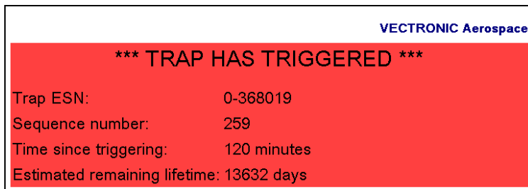
Figure 6: Alarm email
